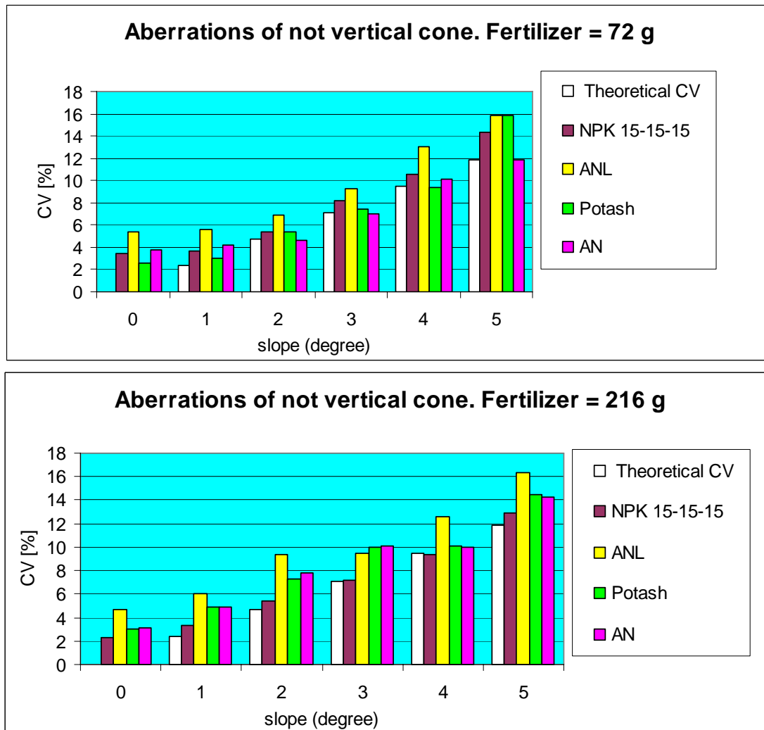
Figure 4: Result of Examination the Cone-belt Dispenser
