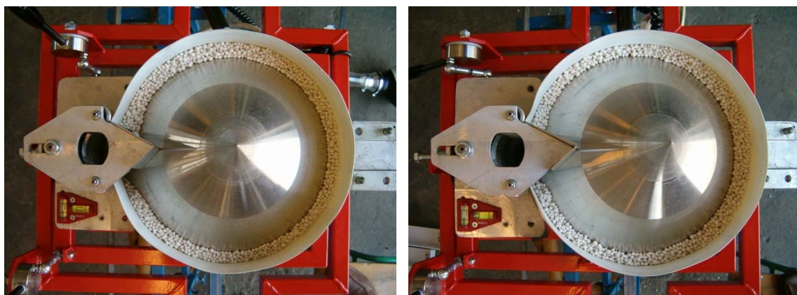
Figure 3: The Fertilizer on the Vertical and on the Not Vertical Cone
